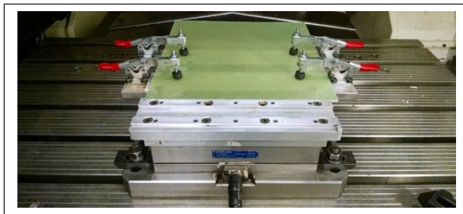
Figure 4 Machining setup
